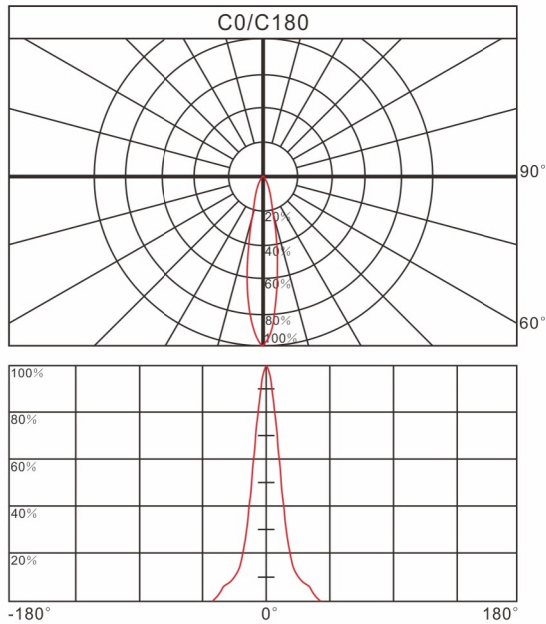
Relative intensity of QR04420
