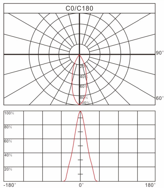
Relative intensity of QR04438
