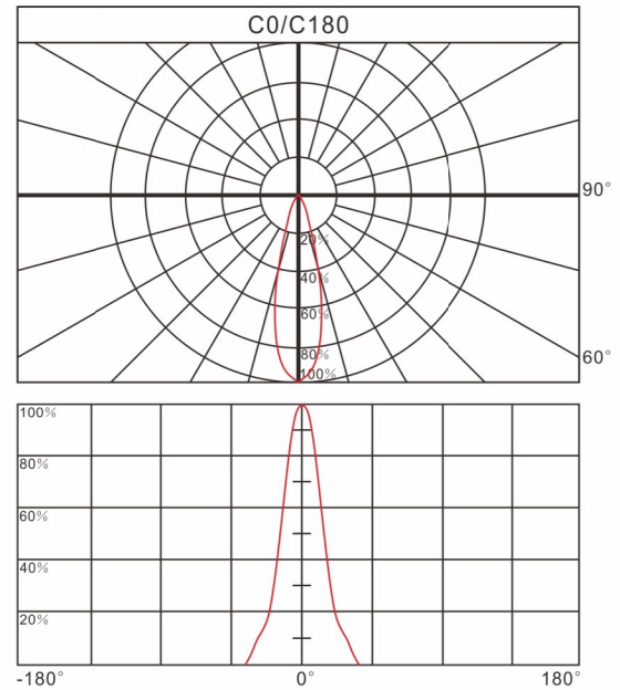
Relative intensity of QR04430
