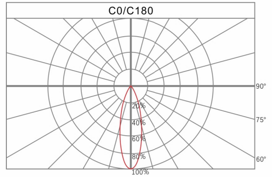
Relative intensity of L03524A-00
