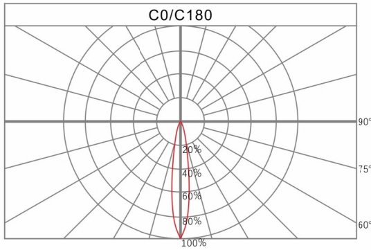
Relative intensity of L03518A-00
