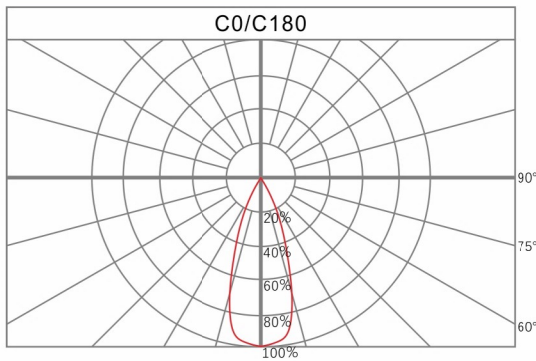
Relative intensity of L03536A-00
