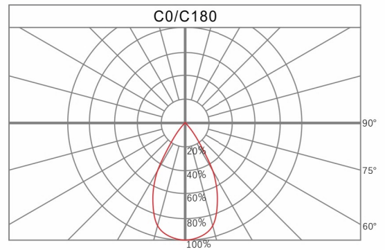
Relative intensity of L03560A-00
